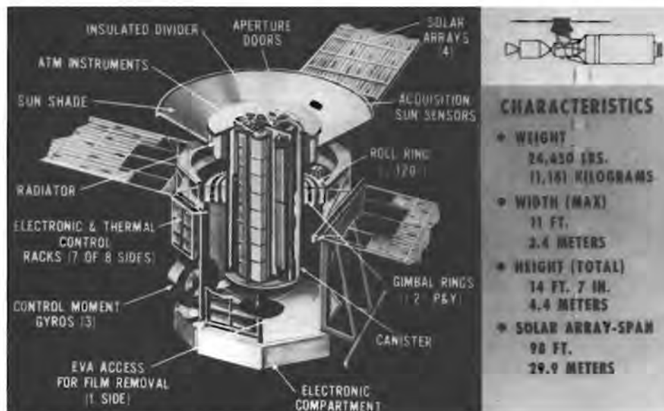
Sketch of the Apollo telescope mount.
