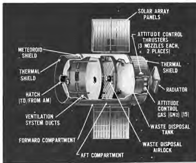
Sketch of the Orbital Workshop.
