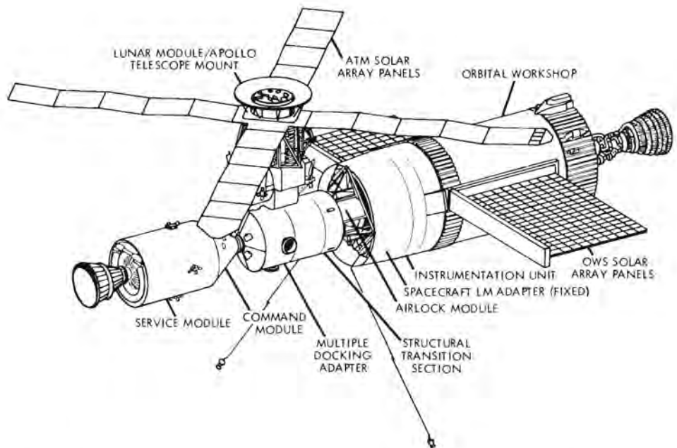
The AAP cluster as visualized by personnel of NASA's Office of Manned Space Flight in Washington in September 1968.
