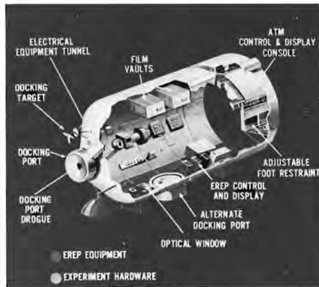
Sketch of the multiple docking adapter.
