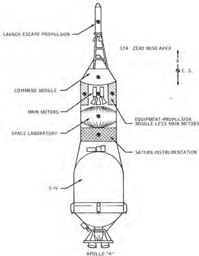
POSSIBLE APOLLO ORBITING LABORATORY
