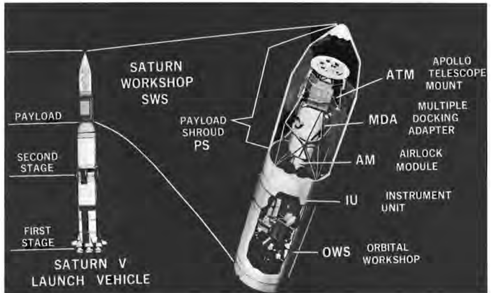
Skylab unmanned launch configurations.
