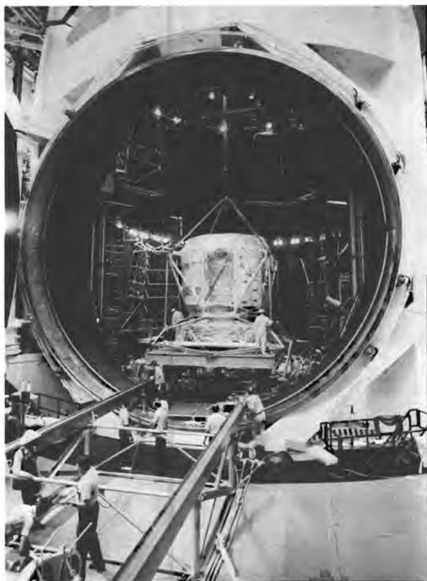
Above, the Apollo telescope mount flight article is shown being placed in the Space Environment Simulation Laboratory chamber at MSC for extensive thermal vacuum testing to verify its ability to withstand the harsh environment of space.
