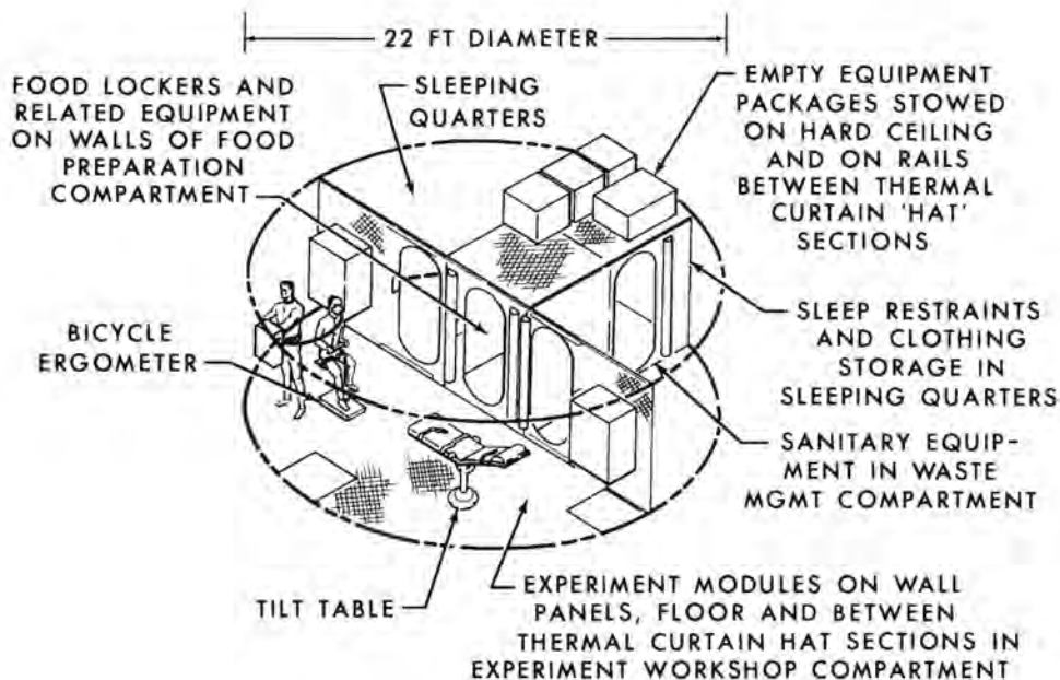
AAP cluster experiments for S-IVB Orbital Workshop.
