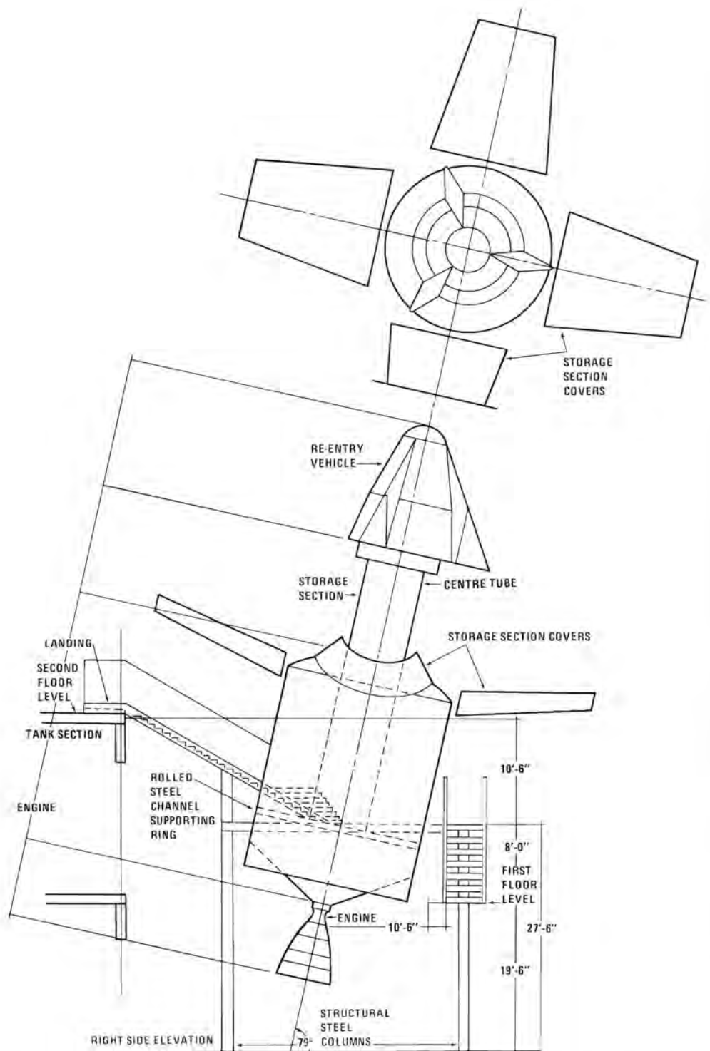
The architectural plans drawn for the 1960 Ideal Home Exhibition in Empire Hall, London, showing three views of the mockup space station.—Drawings courtesy of the London Daily Mail .
