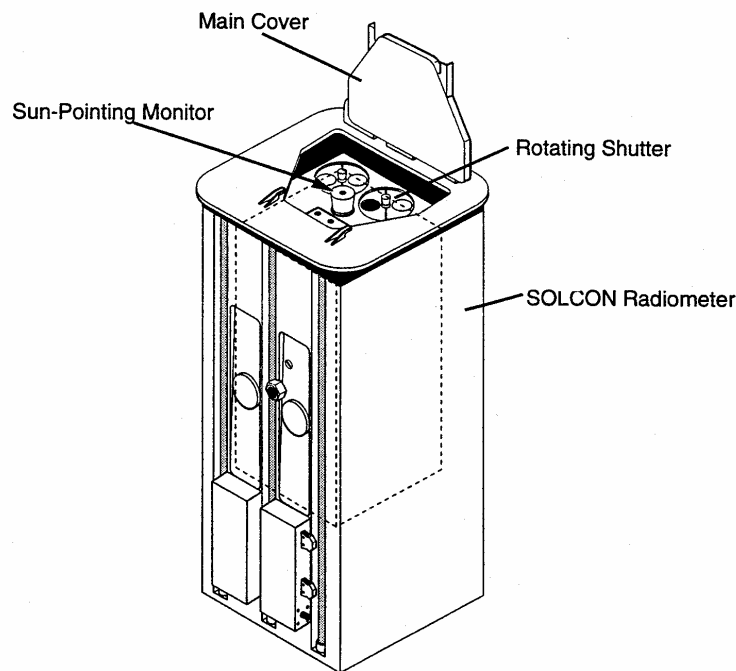
Measurement of the Solar Constant (SOLCON)
