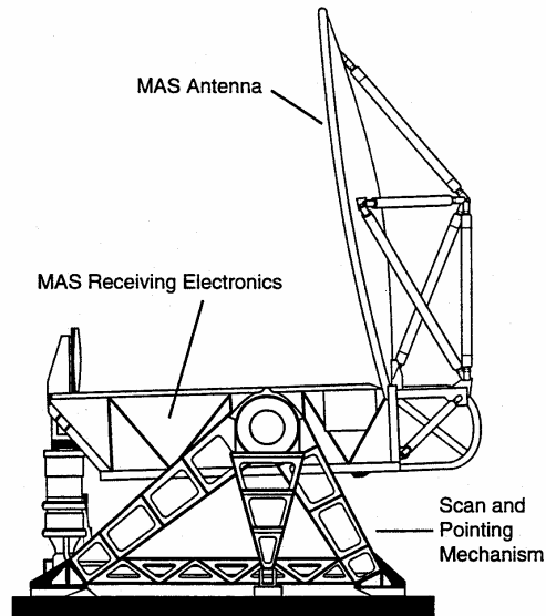
Millimeter-Wave Atmospheric Sounder (MAS)
