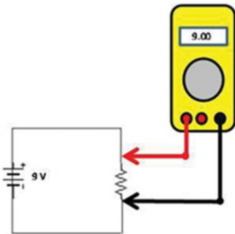
Checking voltage drop across a resistor
