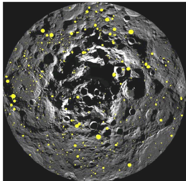
Craters at the lunar South Pole area containing permanent shadow
